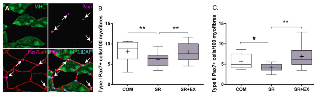
Figure 2 Representative images (A) of single channel stains for myosin heavy chain (MHC)1, and Pax7 and merged stain of Pax7/laminin (LAM) and Pax7/LAM/MHCI/DAPI of a muscle cross section. Scale bar = 50 \mu\text{m} . Quantification of the number of satellite cells (Pax7 + myonuclei/fibre) in type I (B) and type II (C) muscle fibres during step reduction (SR; N = 14 ), step reduction with low-load resistance exercise (SR + EX; N = 14 ), and in healthy ambulatory comparators (COM; N = 7 ). Data presented as mean ('+'), median (line), interquartile range (box), and minimum and maximum (whiskers). **Significantly different, P < 0.01 . #Trend for a difference, P = 0.027 .
